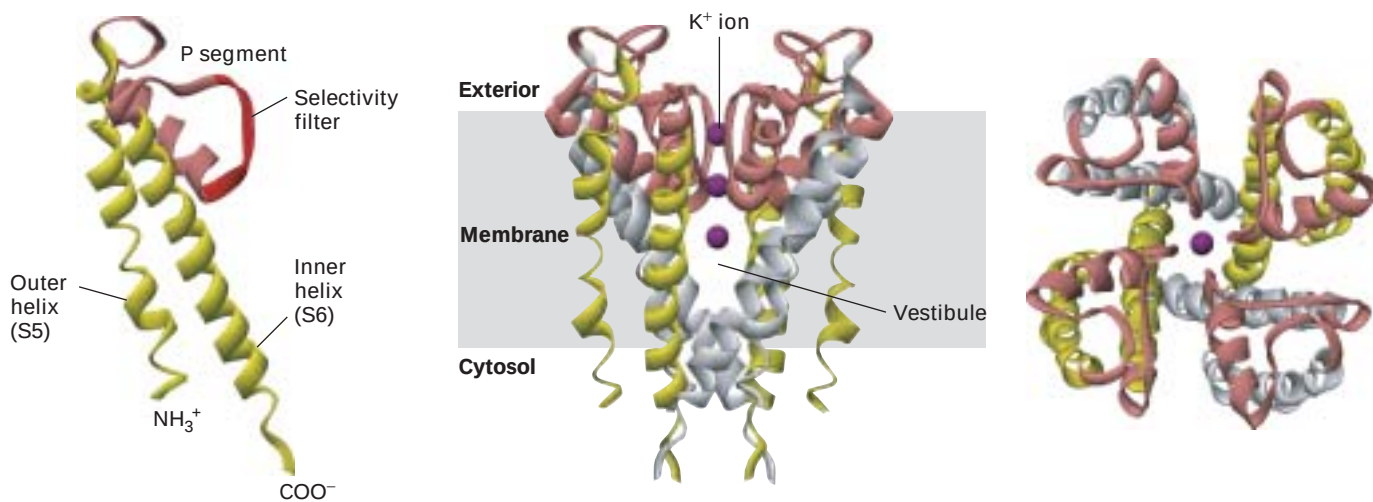
▲ Figure 7-15 Structure of resting K^+ channel from the bacterium Streptomyces lividans . All K^+ channel proteins are tetramers comprising four identical subunits each containing two conserved membrane-spanning \alpha helices, called by convention S5 and S6 (yellow), and a shorter P, or pore segment (pink). (a) One of the subunits, viewed from the side, with key structural features indicated. (b) The complete tetrameric channel viewed from the side (left) and the top, or extracellular, end (right). The P segments are located near the exoplasmic surface and connect the S5 and
