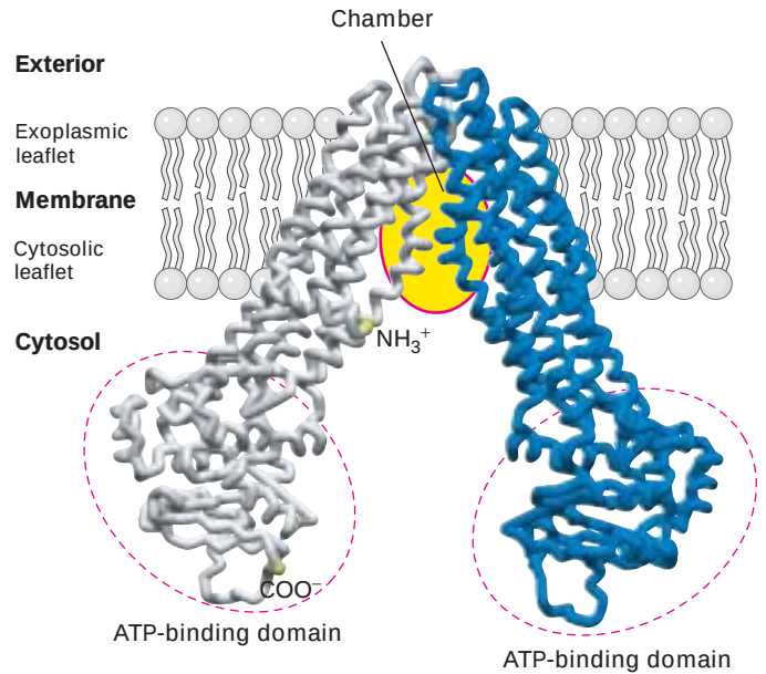
▲ FIGURE 7-11 Structural model of E. coli lipid flippase, an ABC protein homologous to mammalian MDR1. The V-shaped protein encloses a “chamber” within the bilayer where it is hypothesized that bound substrates are flipped across the membrane, as depicted in Figure 7-12. Each identical subunit in this homodimeric protein has one transmembrane domain, comprising six \alpha helices, and one cytosolic domain where ATP binding occurs. [Adapted from G. Chang and C. Roth, 2001, Science 293:1793.]
