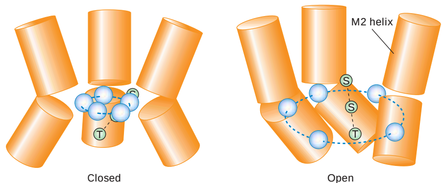
► FIGURE 7-46 Schematic models of the pore-lining M2 helices in the closed and opened states. In the closed state, the kink in the center of each M2 helix points inward, constricting the passageway, whose perimeter is indicated by the blue spheres. In the open state, the kinks rotate to one side, so that the helices are farther apart. The green spheres denote the hydroxyl groups of serine (S) and threonine (T) residues in the center of the M2 helices; in the open state these are parallel to the channel axis and allow ions to flow.
