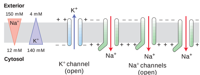
▲ FIGURE 7-32 Depolarization of the plasma membrane due to opening of gated Na^+ channels. (a) In resting neurons, nongated K^+ channels are open, but the more numerous gated Na^+ channels are closed. The movement of K^+ ions outward establishes the inside-negative membrane potential characteristic of most cells. (b) Opening of gated Na^+ channels permits an influx of sufficient Na^+ ions to cause a reversal of the membrane potential. See text for details.
